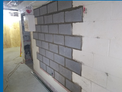
In-fill of Masonry Walls.
